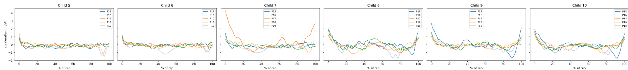
Bench Press — z_accel
